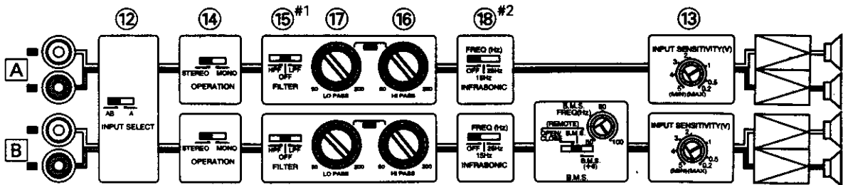
Block diagram
